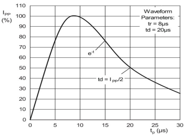
Figure3. Pulse Waveform
