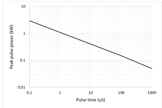
Figure2. Peak Pulse Power vs. Pulse Time
